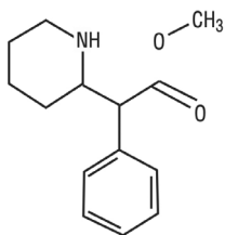
Figure 1: Methylphenidate Structure
